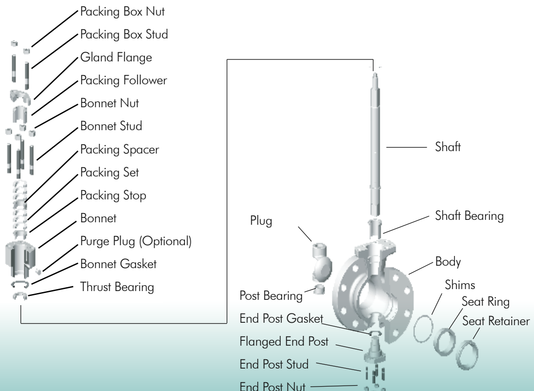
Figure 2: Exploded View
