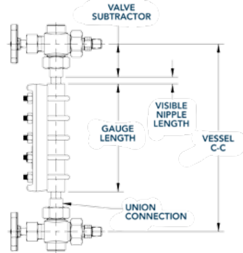
End Connected Gauge with KMVU/KHVV Valves
