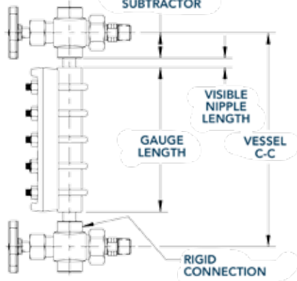
End Connected Gauge with KMVR/KHVR Valves
