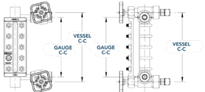
Side Connected Gauges with Valve C-C Mounted Outside Gauge C-C (Figure 2) To find gauge C-C, subtract 1.50" from vessel C-C
