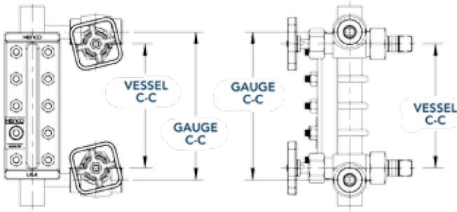
Side Connected Gauges with Valve C-C Mounted Inside Gauge C-C (Figure 1) To find gauge C-C, add 1.50" to vessel C-C
